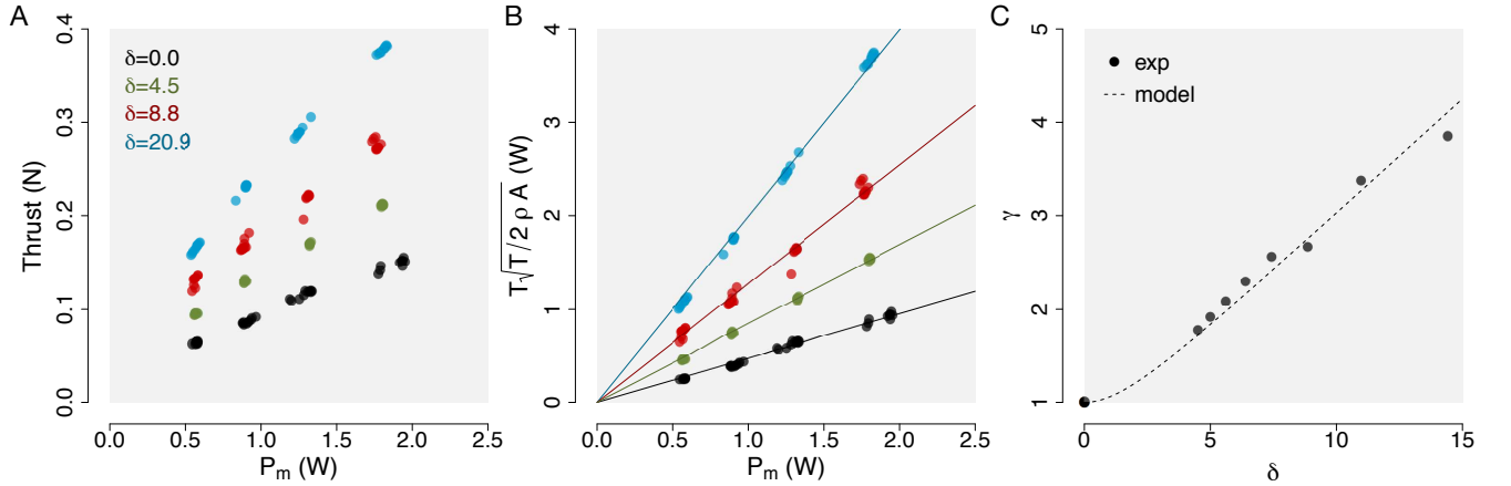
Fig. 5. (A) The plot of mechanical power against the thrust force. (B) The relationship between P_m and T/\sqrt{T/2\rho A} is linear as predicted. (C) The ceiling coefficients deduced from the experimental data at different propeller-to-ceiling ratios follows the trend predicted by the model with the correction factor \alpha = 2.0 .
